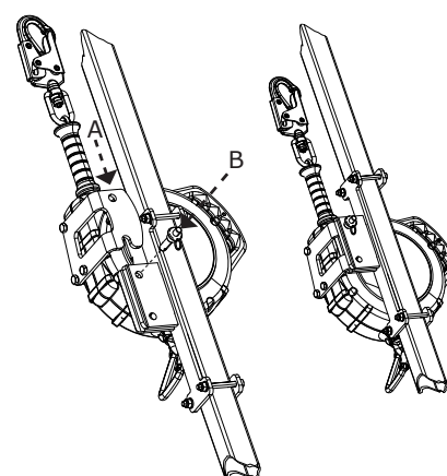
Figure 4 - Mount SRL on Protecta Tripod Mating Bracket
