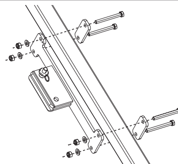
Figure 3 - Install Mounting Bracket on SRL
